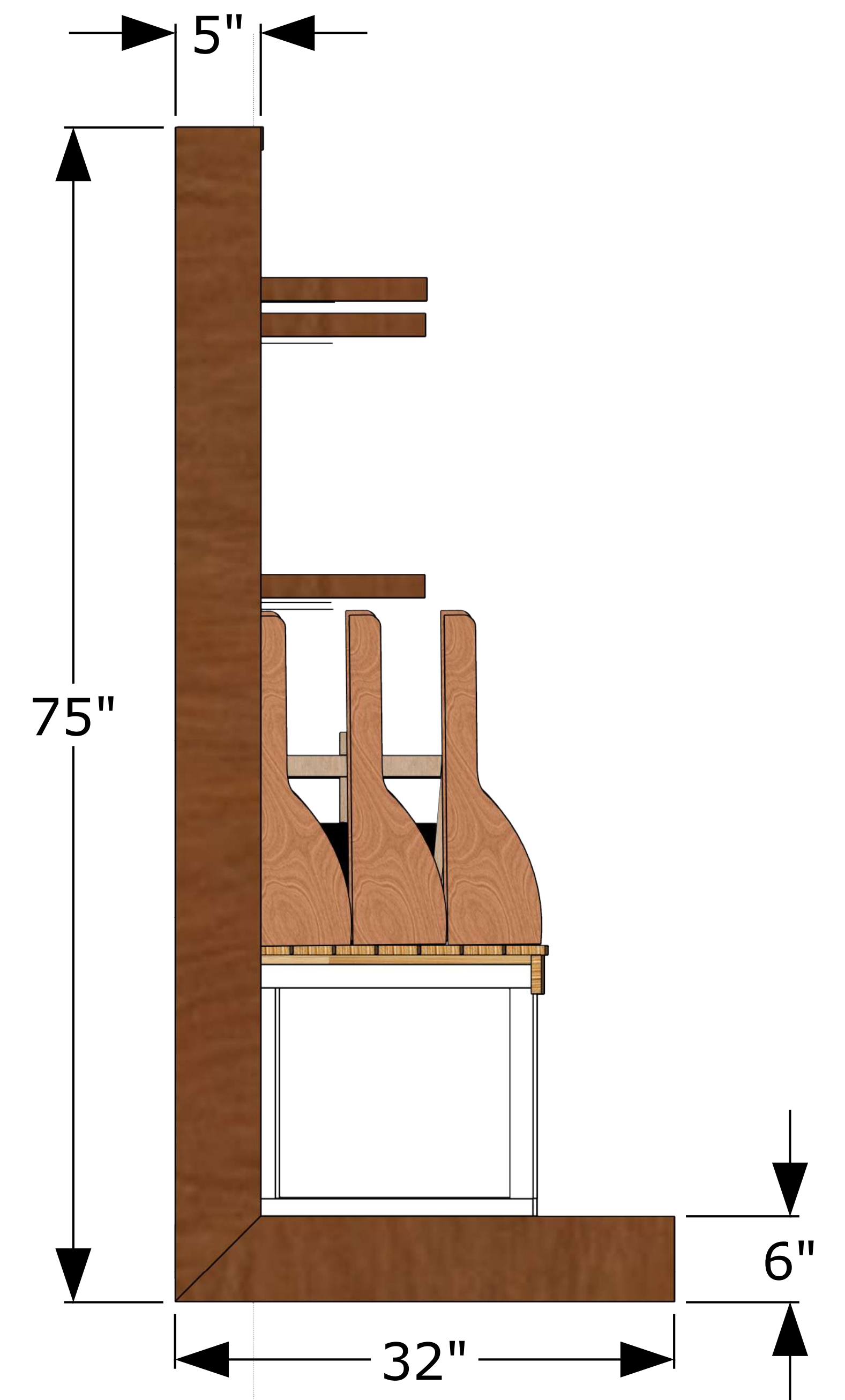
Side View
