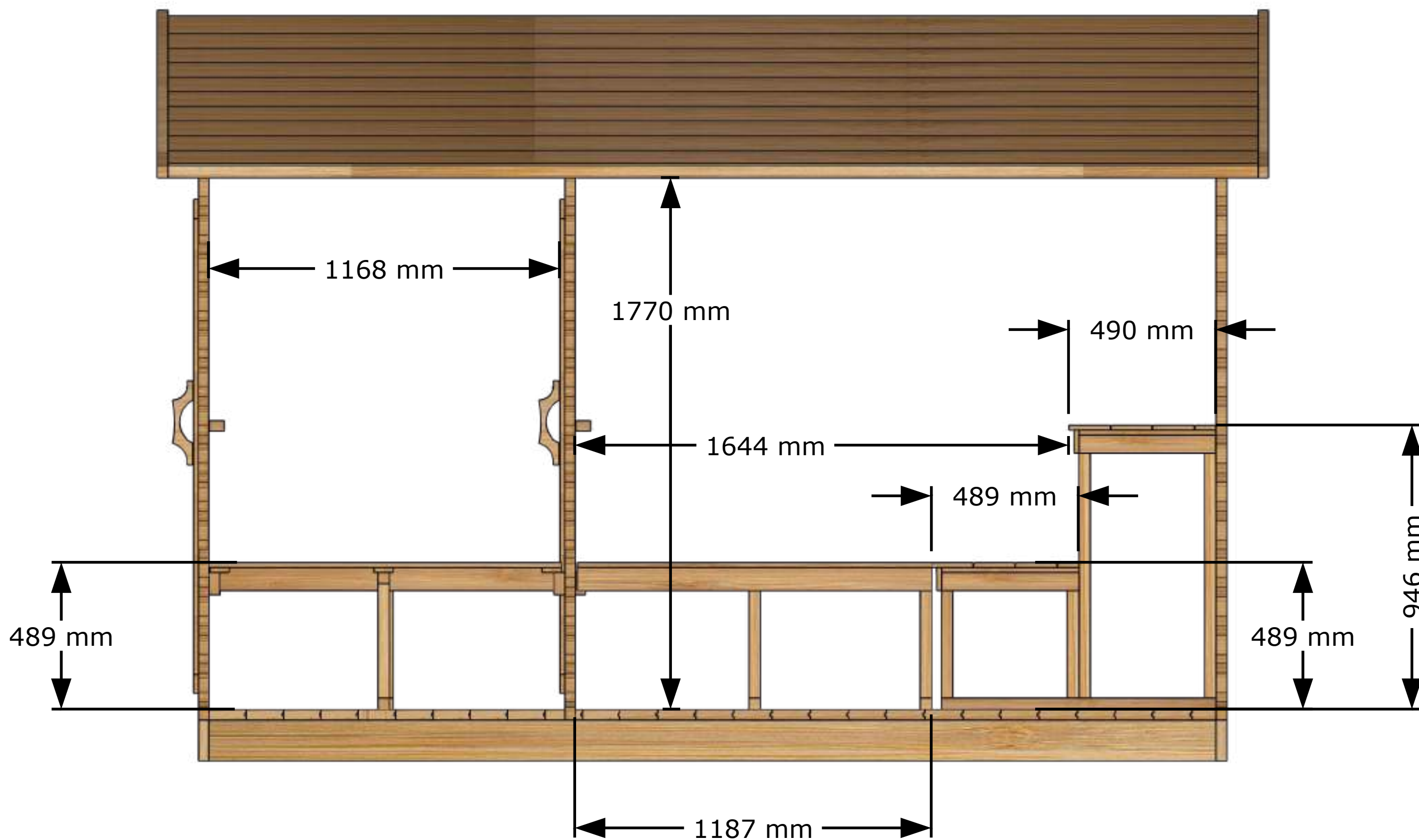
Side View
