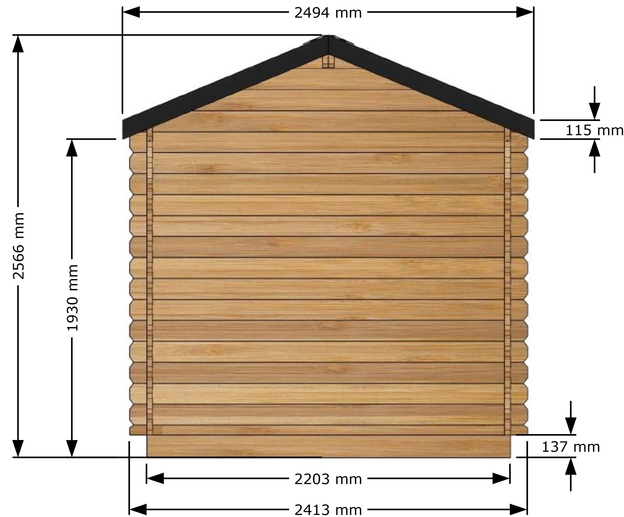
Side View
