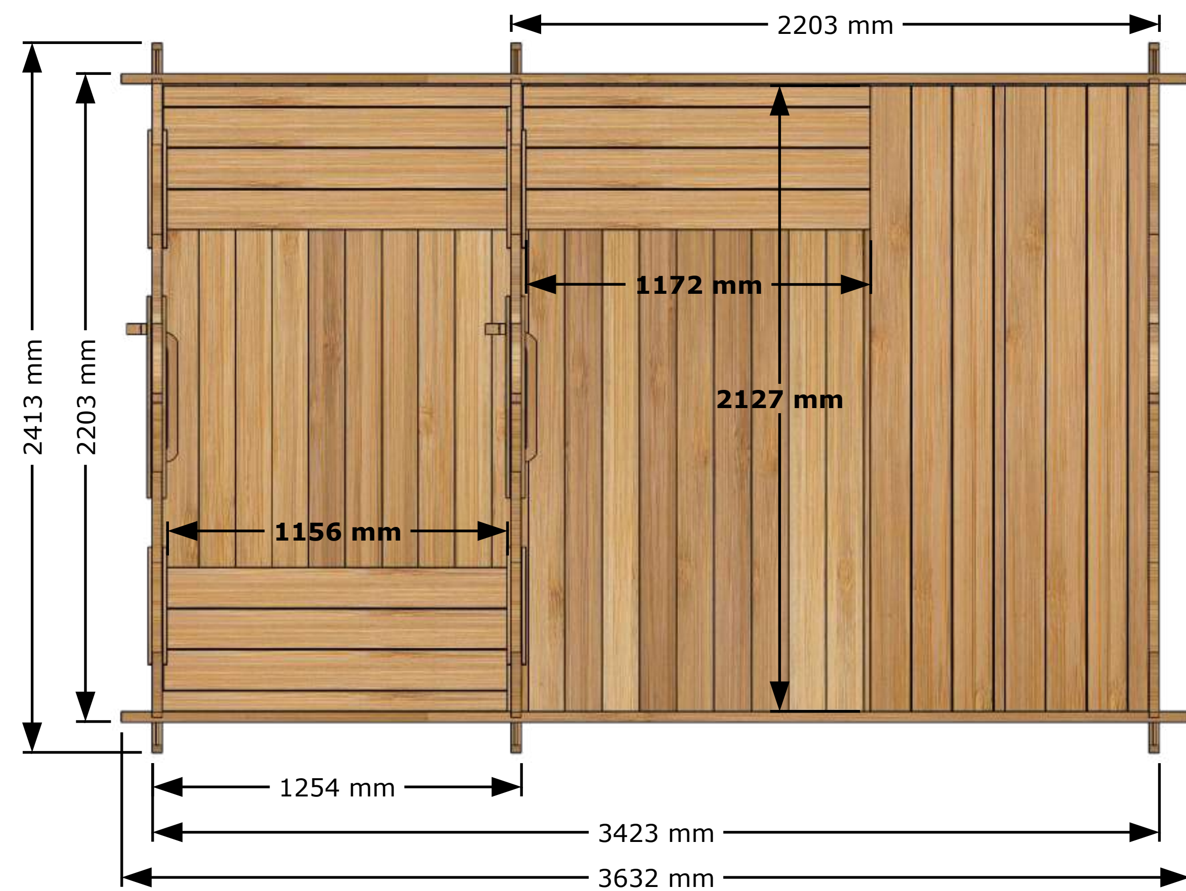
Top View
