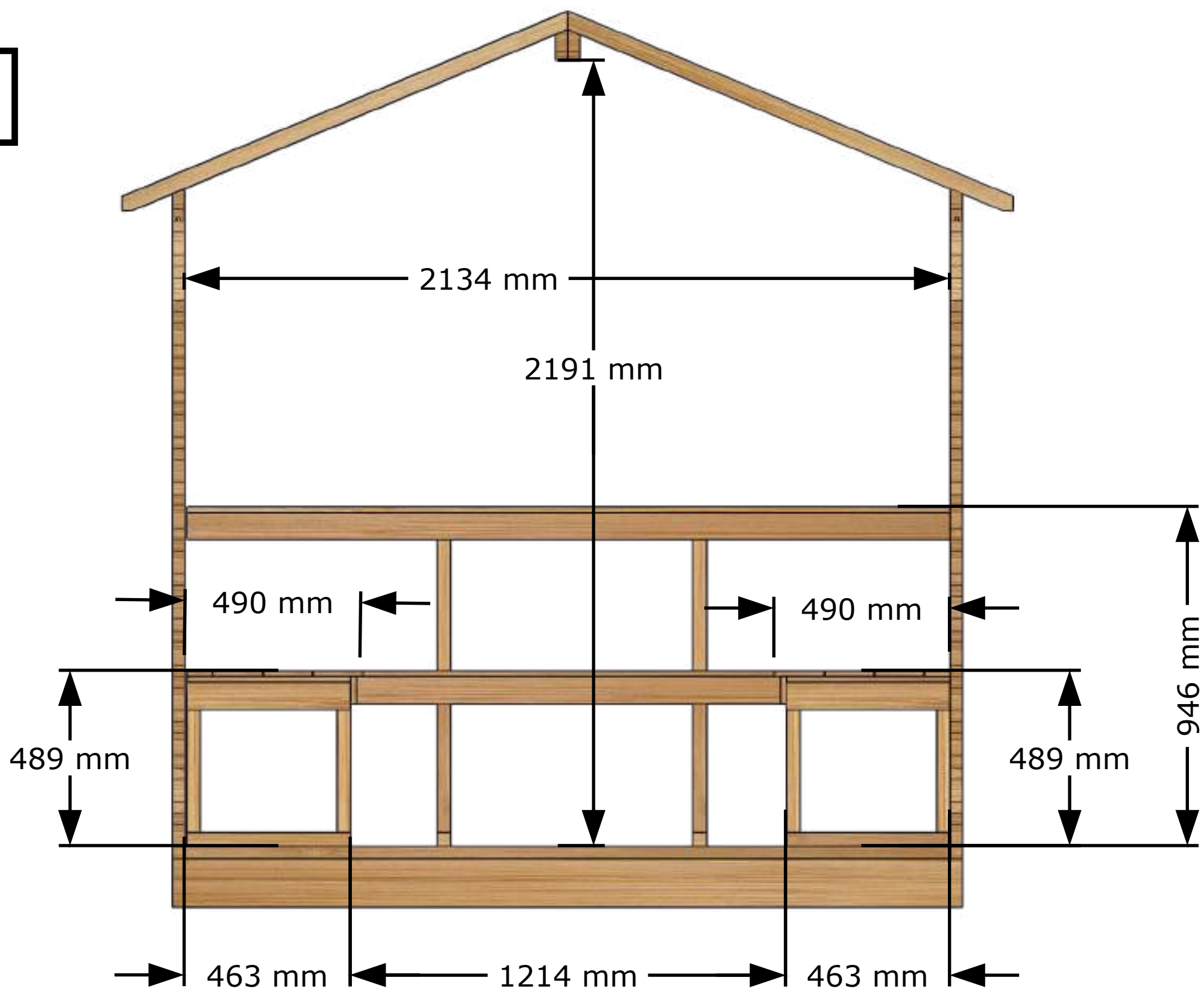
Front View
